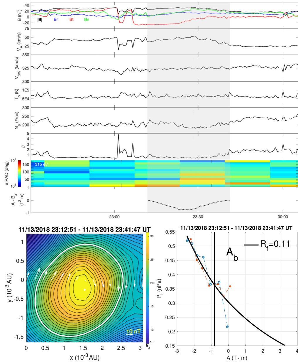
Figure 5. from Small-scale Magnetic Flux Ropes in the First Two Parker Solar Probe Encounters null 2020 APJ 903 76 doi:10.3847/1538-4357/abb820 https://dx.doi.org/10.3847/1538-4357/abb820
