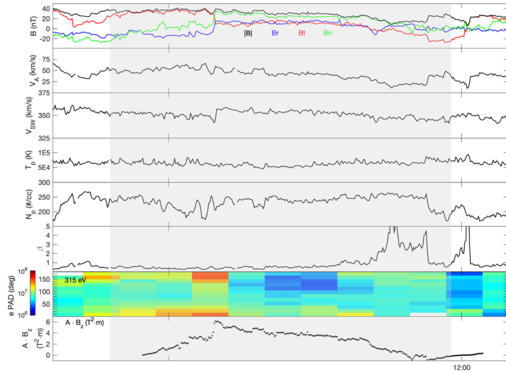
Figure 4. from Small-scale Magnetic Flux Ropes in the First Two Parker Solar Probe Encounters null 2020 APJ 903 76 doi:10.3847/1538-4357/abb820 https://dx.doi.org/10.3847/1538-4357/abb820 © 2020. The American Astronomical Society. All rights reserved.
