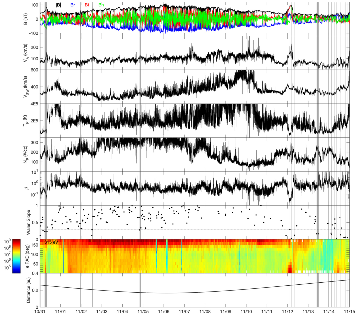
Figure 1. from Small-scale Magnetic Flux Ropes in the First Two Parker Solar Probe Encounters null 2020 APJ 903 76 doi:10.3847/1538-4357/abb820 https://dx.doi.org/10.3847/1538-4357/abb820 © 2020. The American Astronomical Society. All rights reserved.
