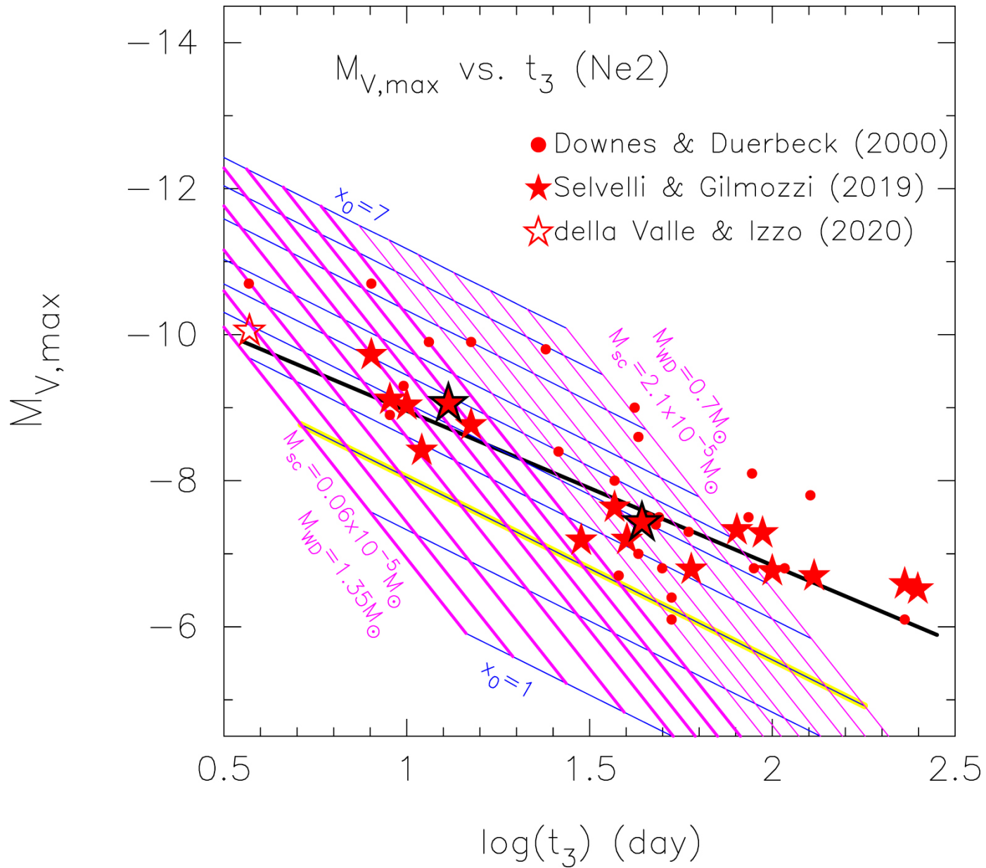
Figure 9. from A Theory for the Maximum Magnitude versus Rate of Decline Relation of Classical Novae null 2020 APJ 902 91 doi:10.3847/1538-4357/abb5fa https://dx.doi.org/10.3847/1538-4357/abb5fa © 2020. The American Astronomical Society. All rights reserved.
