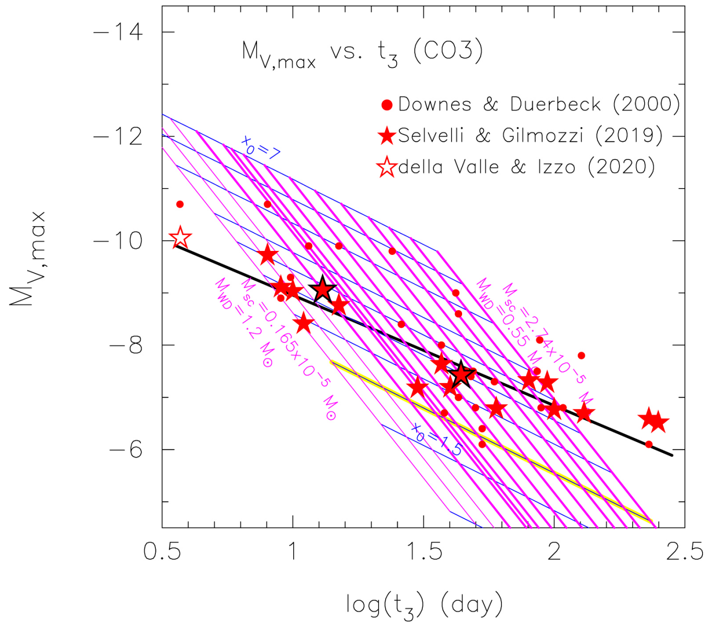
Figure 8. from A Theory for the Maximum Magnitude versus Rate of Decline Relation of Classical Novae null 2020 APJ 902 91 doi:10.3847/1538-4357/abb5fa https://dx.doi.org/10.3847/1538-4357/abb5fa © 2020. The American Astronomical Society. All rights reserved.
