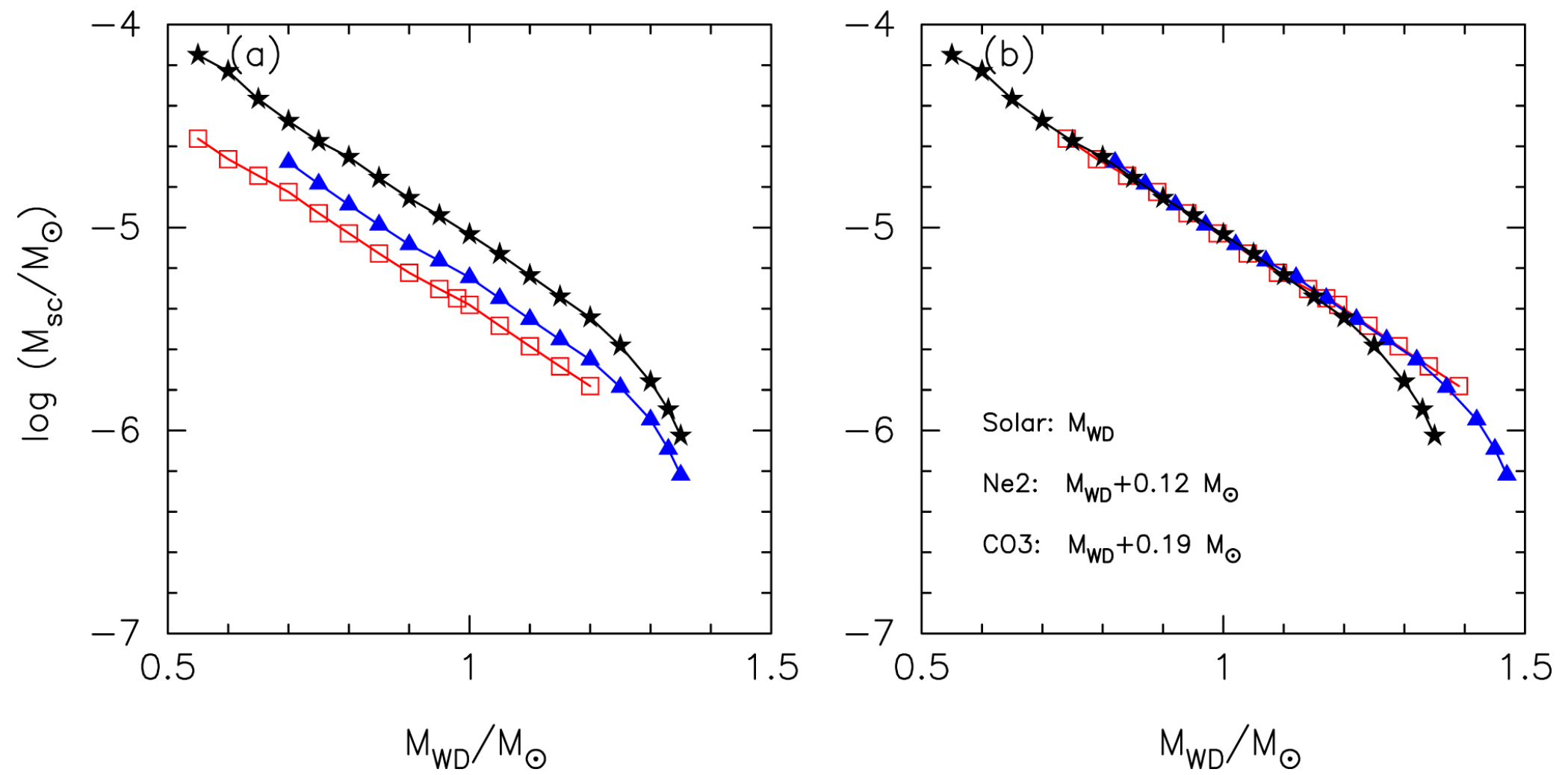
Figure 7. from A Theory for the Maximum Magnitude versus Rate of Decline Relation of Classical Novae null 2020 APJ 902 91 doi:10.3847/1538-4357/abb5fa https://dx.doi.org/10.3847/1538-4357/abb5fa © 2020. The American Astronomical Society. All rights reserved.
