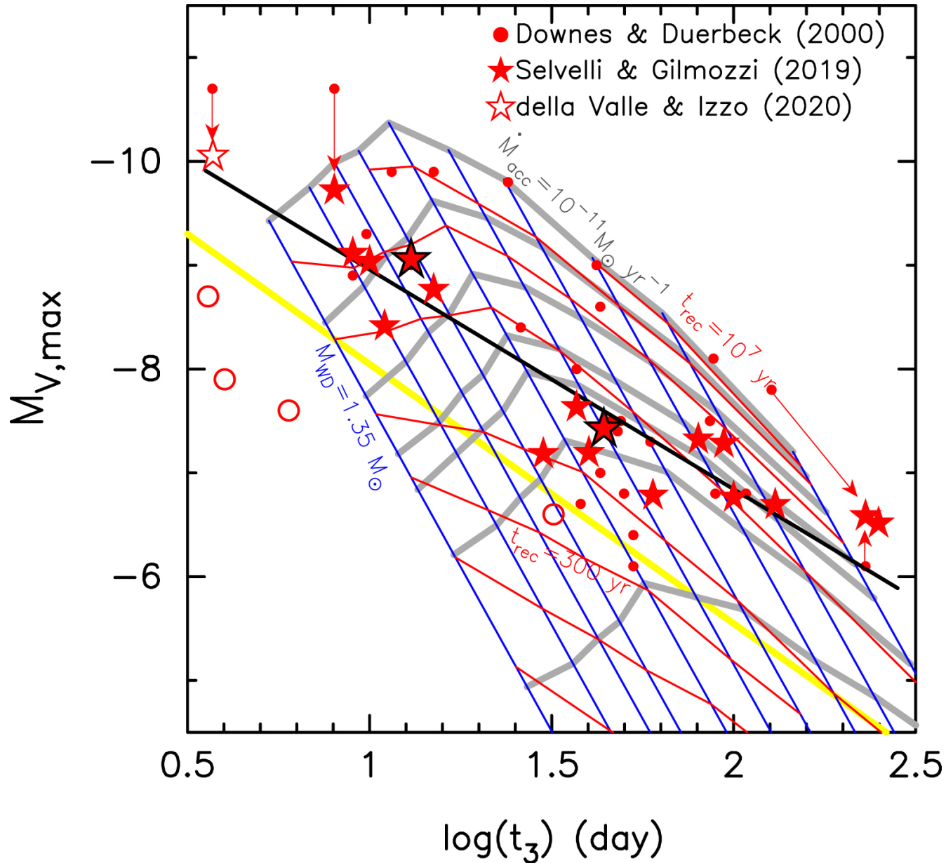
Figure 6. from A Theory for the Maximum Magnitude versus Rate of Decline Relation of Classical Novae null 2020 APJ 902 91 doi:10.3847/1538-4357/abb5fa https://dx.doi.org/10.3847/1538-4357/abb5fa © 2020. The American Astronomical Society. All rights reserved.
