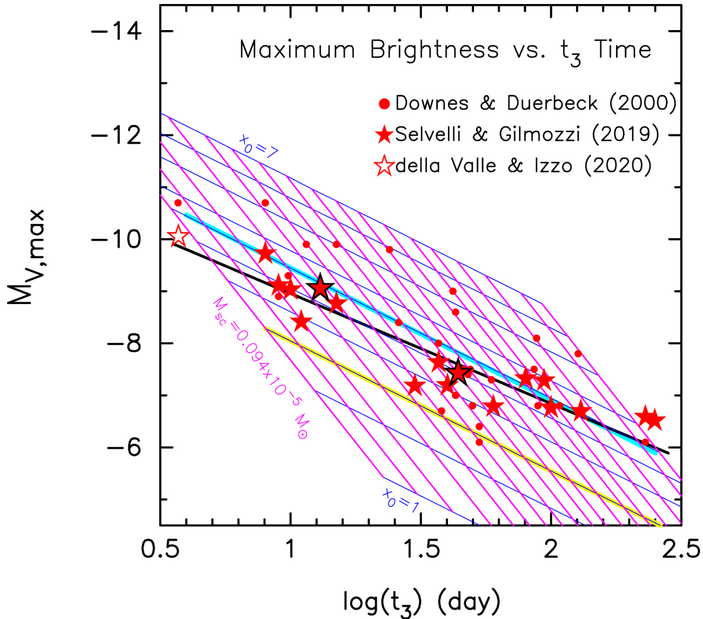
Figure 5. from A Theory for the Maximum Magnitude versus Rate of Decline Relation of Classical Novae null 2020 APJ 902 91 doi:10.3847/1538-4357/abb5fa https://dx.doi.org/10.3847/1538-4357/abb5fa © 2020. The American Astronomical Society. All rights reserved.
