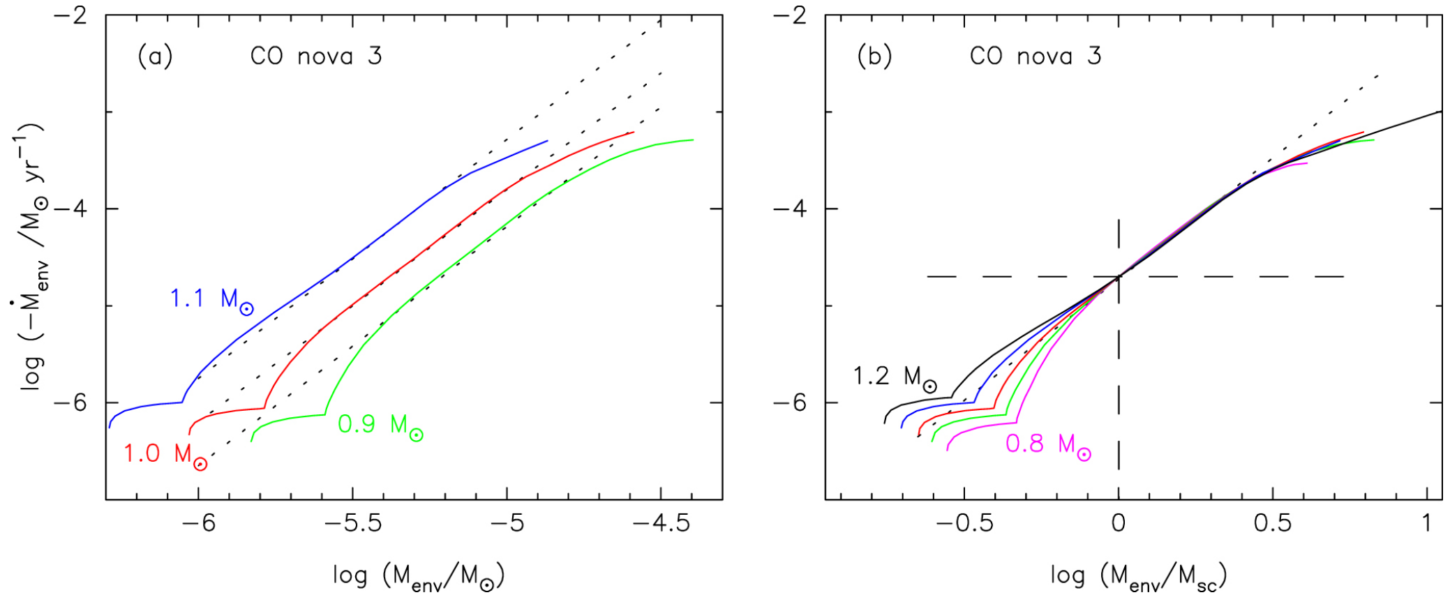
Figure 3. from A Theory for the Maximum Magnitude versus Rate of Decline Relation of Classical Novae null 2020 APJ 902 91 doi:10.3847/1538-4357/abb5fa https://dx.doi.org/10.3847/1538-4357/abb5fa © 2020. The American Astronomical Society. All rights reserved.
