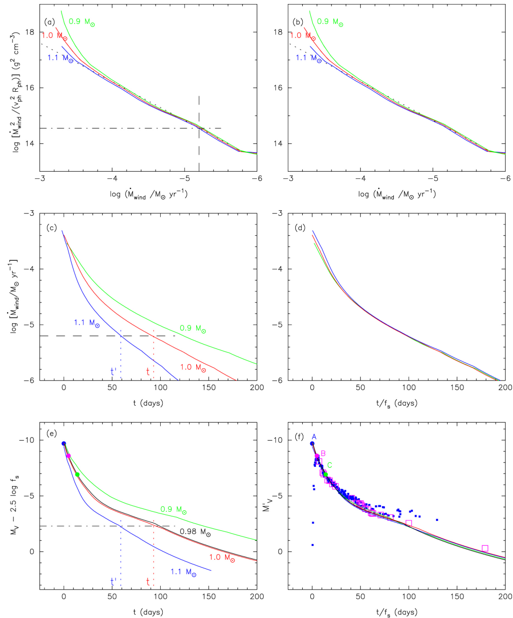
Figure 2. from A Theory for the Maximum Magnitude versus Rate of Decline Relation of Classical Novae null 2020 APJ 902 91 doi:10.3847/1538-4357/abb5fa https://dx.doi.org/10.3847/1538-4357/abb5fa © 2020. The American Astronomical Society. All rights reserved.
