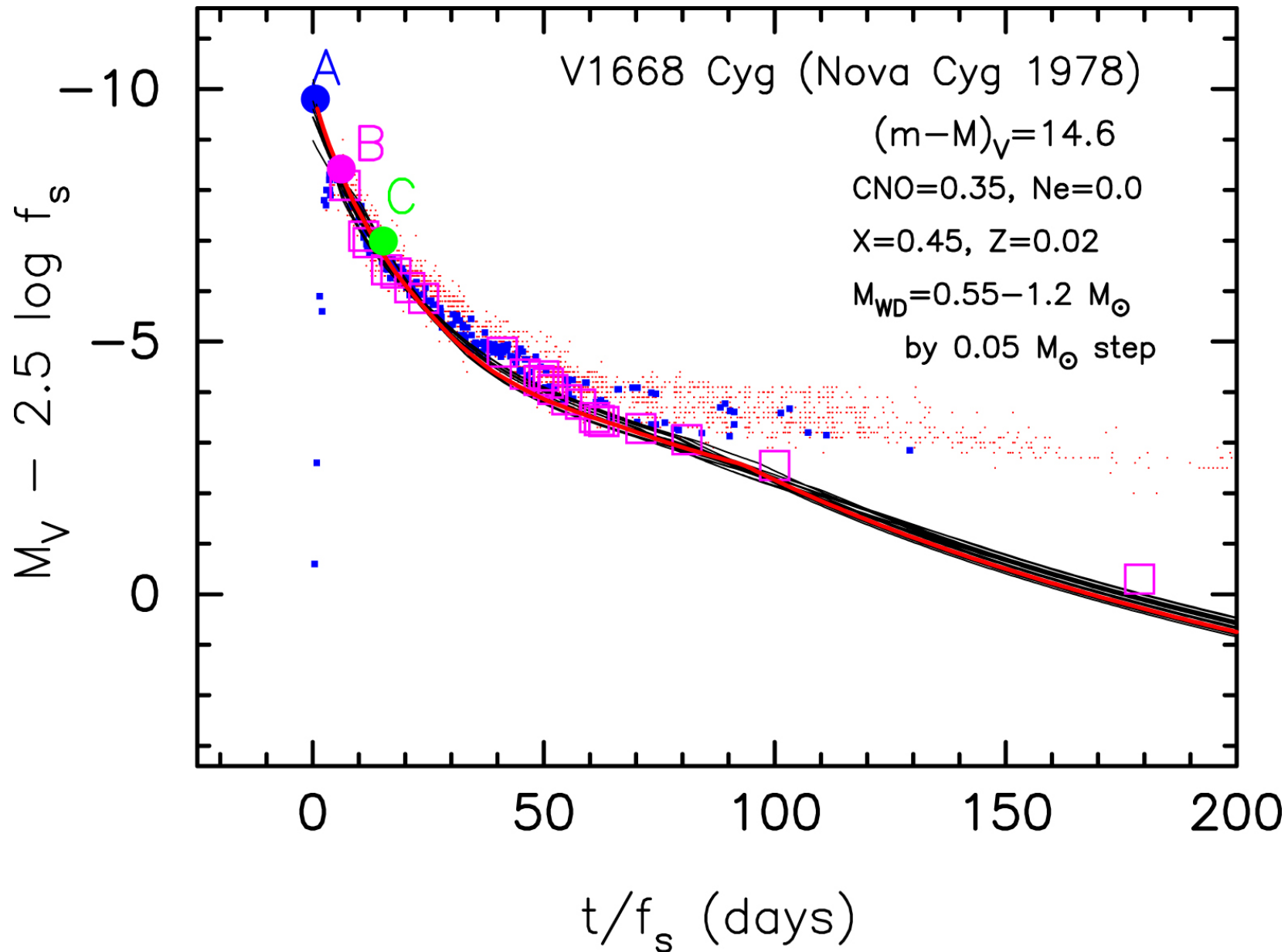
Figure 1. from A Theory for the Maximum Magnitude versus Rate of Decline Relation of Classical Novae null 2020 APJ 902 91 doi:10.3847/1538-4357/abb5fa https://dx.doi.org/10.3847/1538-4357/abb5fa © 2020. The American Astronomical Society. All rights reserved.
