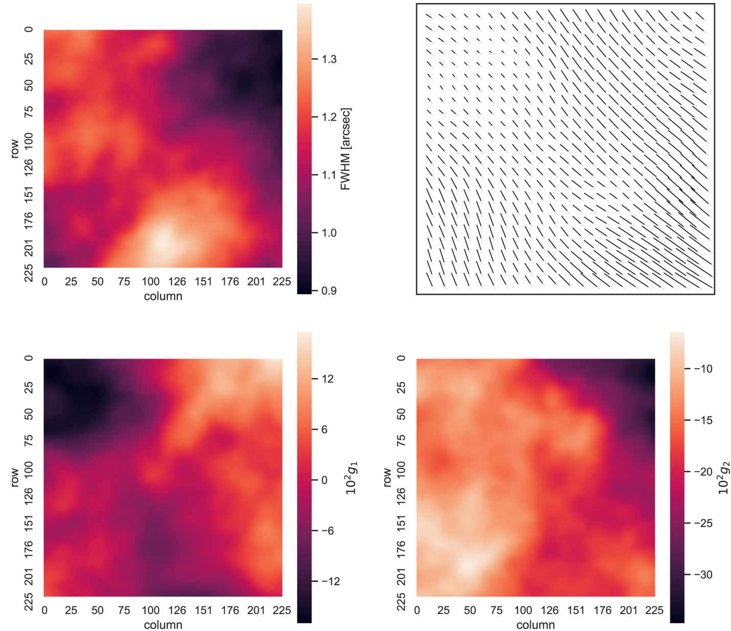
Figure A1. from Mitigating Shear-dependent Object Detection Biases with Metacalibration null 2020 APJ 902 138 doi:10.3847/1538-4357/abb595 https://dx.doi.org/10.3847/1538-4357/abb595 © 2020. The American Astronomical Society. All rights reserved.
