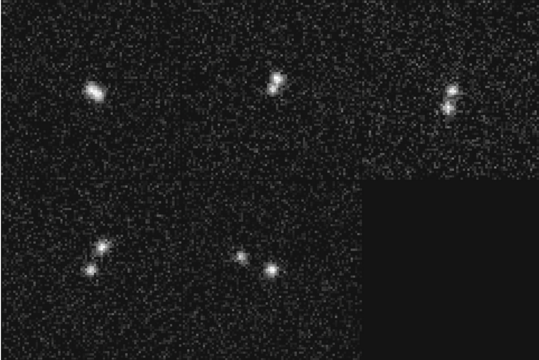
Figure 2. from Mitigating Shear-dependent Object Detection Biases with Metacalibration null 2020 APJ 902 138 doi:10.3847/1538-4357/abb595 https://dx.doi.org/10.3847/1538-4357/abb595 © 2020. The American Astronomical Society. All rights reserved.
