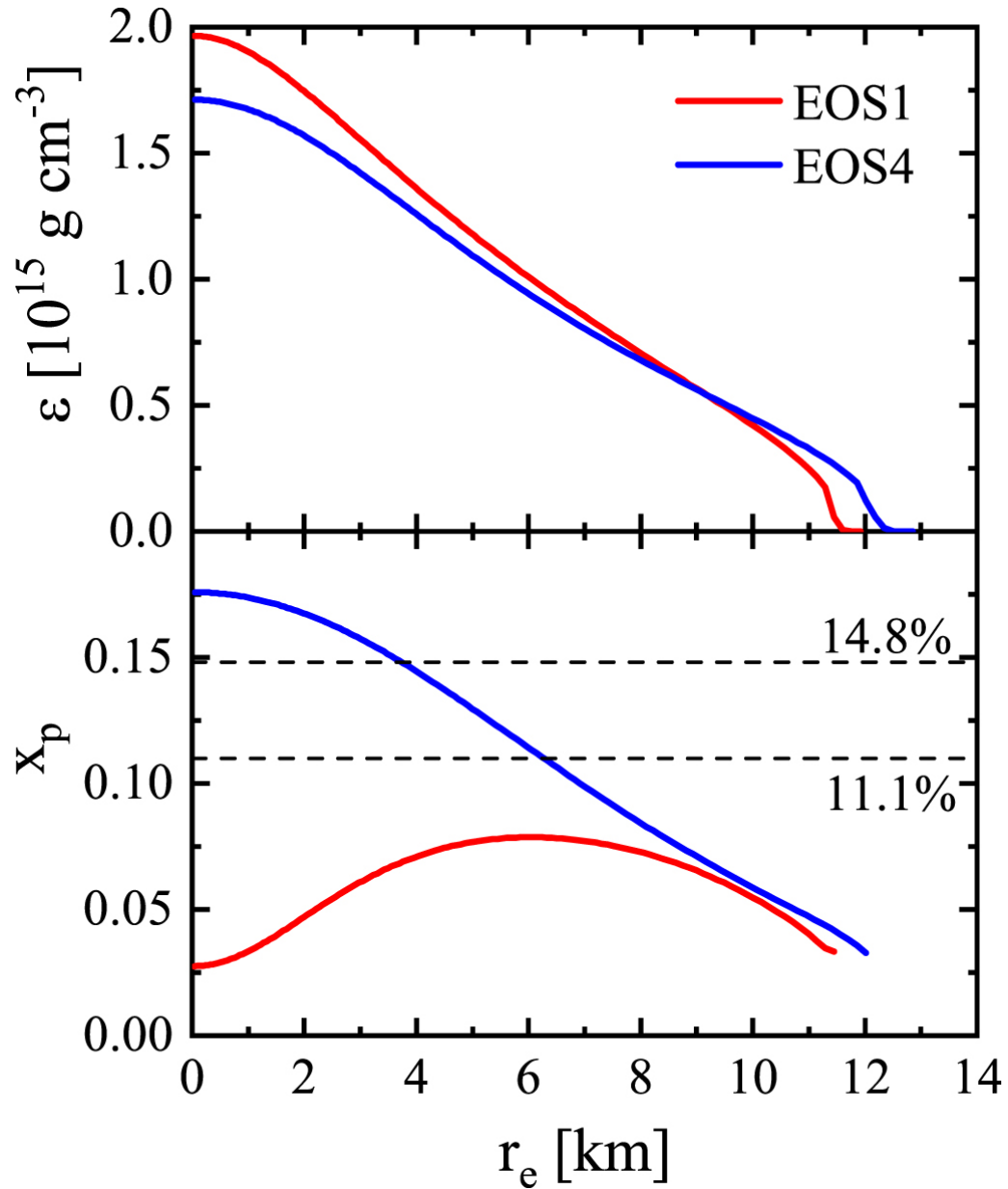
Figure 9. from GW190814's Secondary Component with Mass 2.50–2.67 M as a Superfast Pulsar null 2020 APJ 902 38 doi:10.3847/1538-4357/abb470 https://dx.doi.org/10.3847/1538-4357/abb470 © 2020. The American Astronomical Society. All rights reserved.
