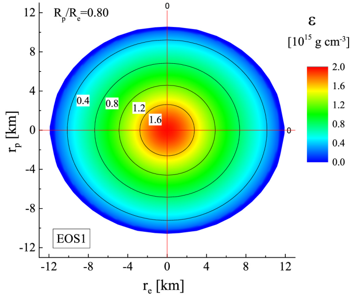
Figure 8. from GW190814's Secondary Component with Mass 2.50–2.67 M as a Superfast Pulsar null 2020 APJ 902 38 doi:10.3847/1538-4357/abb470 https://dx.doi.org/10.3847/1538-4357/abb470
