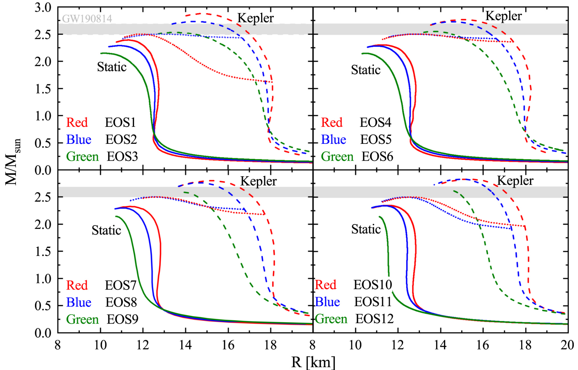
Figure 6. from GW190814's Secondary Component with Mass 2.50–2.67 M as a Superfast Pulsar null 2020 APJ 902 38 doi:10.3847/1538-4357/abb470 https://dx.doi.org/10.3847/1538-4357/abb470
