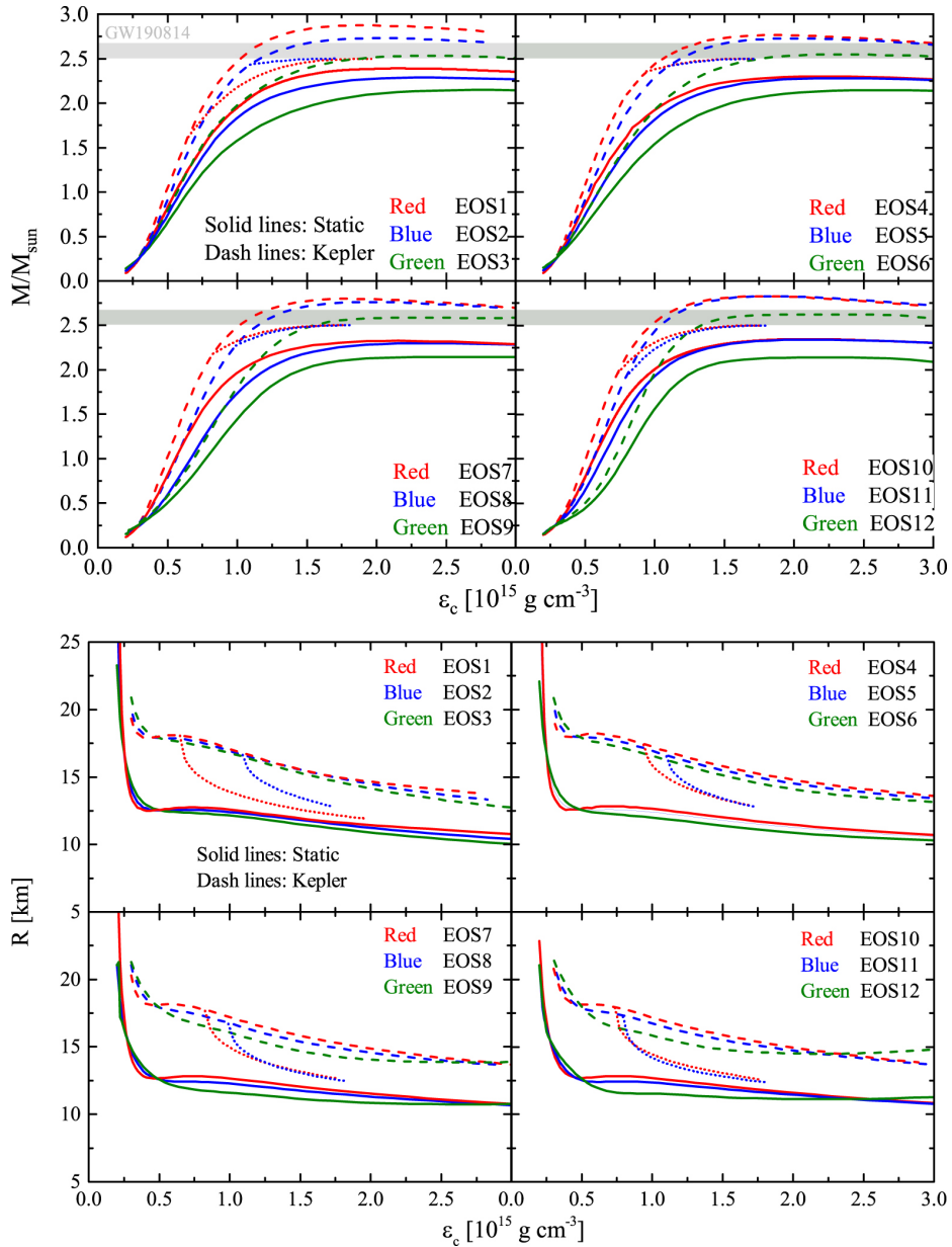
Figure 5. from GW190814's Secondary Component with Mass 2.50–2.67 M as a Superfast Pulsar null 2020 APJ 902 38 doi:10.3847/1538-4357/abb470 https://dx.doi.org/10.3847/1538-4357/abb470
