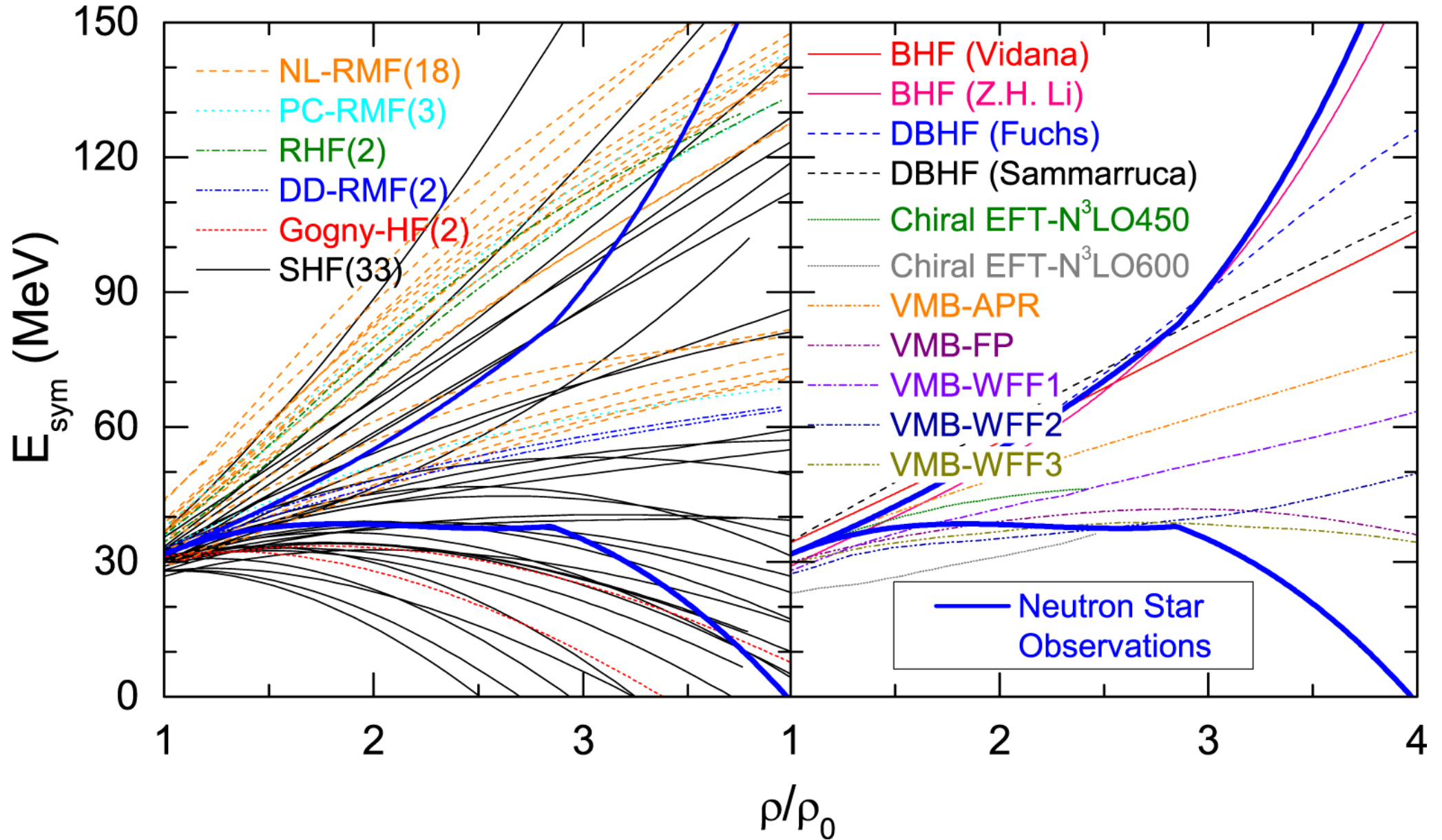
Figure 4. from GW190814's Secondary Component with Mass 2.50–2.67 M as a Superfast Pulsar null 2020 APJ 902 38 doi:10.3847/1538-4357/abb470 https://dx.doi.org/10.3847/1538-4357/abb470 © 2020. The American Astronomical Society. All rights reserved.
