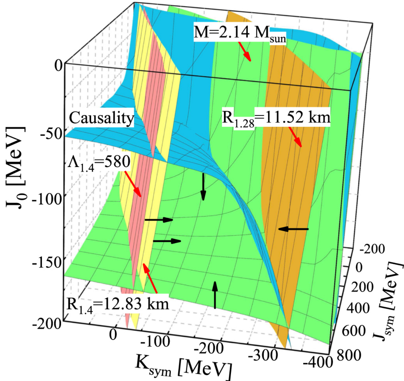
Figure 2. from GW190814's Secondary Component with Mass 2.50–2.67 M as a Superfast Pulsar null 2020 APJ 902 38 doi:10.3847/1538-4357/abb470 https://dx.doi.org/10.3847/1538-4357/abb470 © 2020. The American Astronomical Society. All rights reserved.
