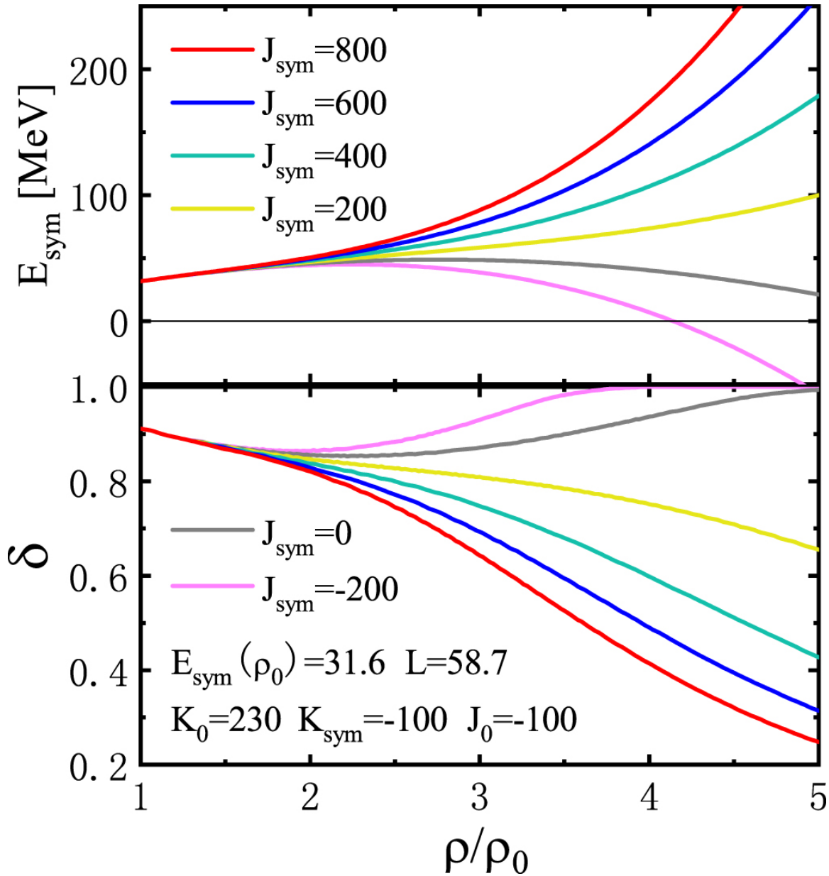
Figure 1. from GW190814's Secondary Component with Mass 2.50–2.67 M as a Superfast Pulsar null 2020 APJ 902 38 doi:10.3847/1538-4357/abb470 https://dx.doi.org/10.3847/1538-4357/abb470 © 2020. The American Astronomical Society. All rights reserved.
