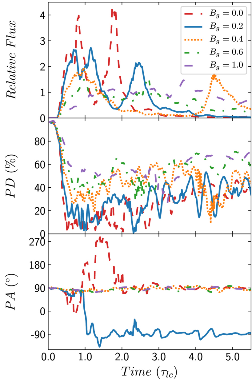
Figure 7. from Radiation and Polarization Signatures from Magnetic Reconnection in Relativistic Jets. I. A Systematic Study null 2020 APJ 901 149 doi:10.3847/1538-4357/abb1b0 https://dx.doi.org/10.3847/1538-4357/abb1b0 © 2020. The American Astronomical Society. All rights reserved.
