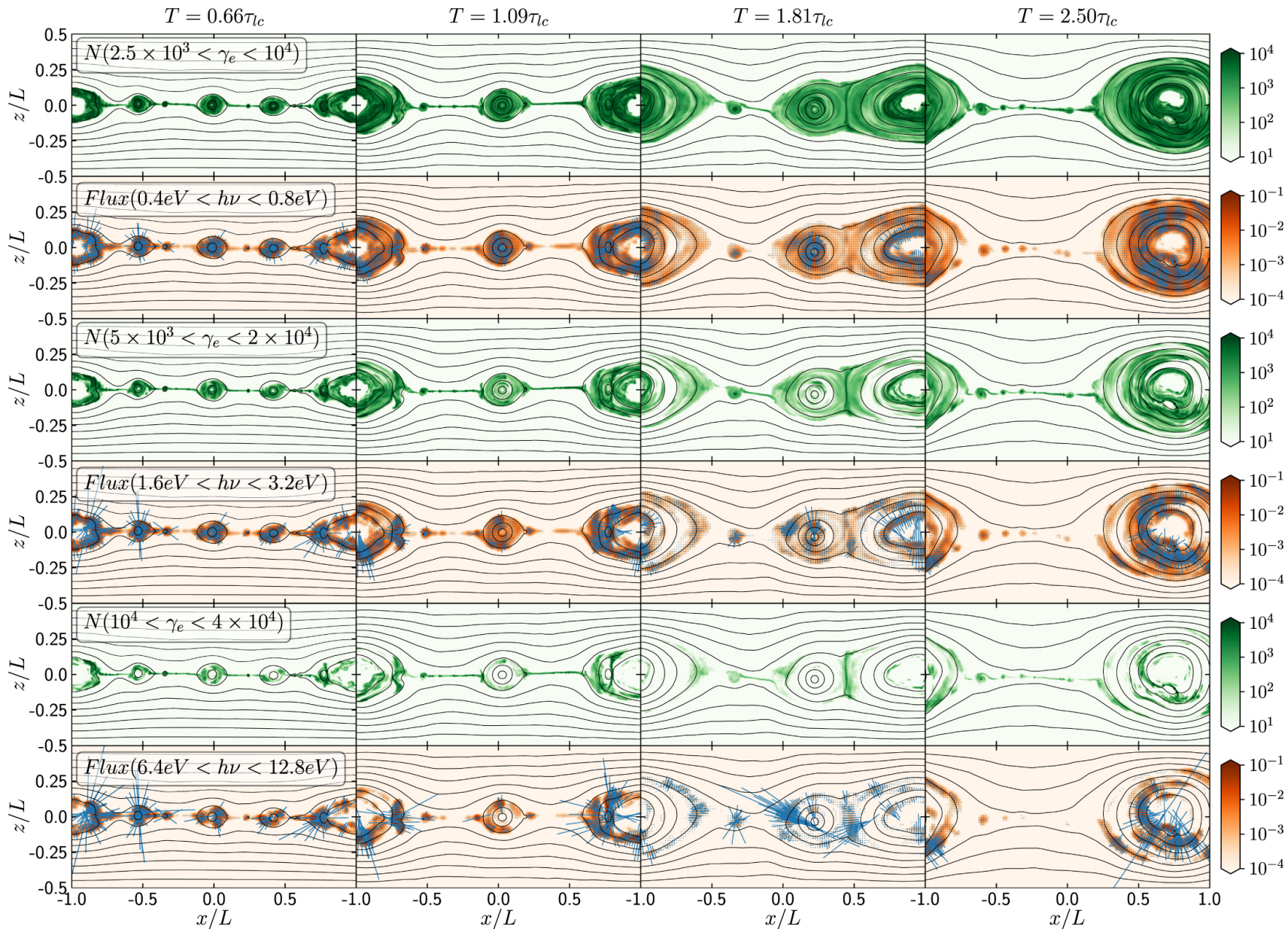
Figure 6. from Radiation and Polarization Signatures from Magnetic Reconnection in Relativistic Jets. I. A Systematic Study null 2020 APJ 901 149 doi:10.3847/1538-4357/abb1b0 https://dx.doi.org/10.3847/1538-4357/abb1b0 © 2020. The American Astronomical Society. All rights reserved.
