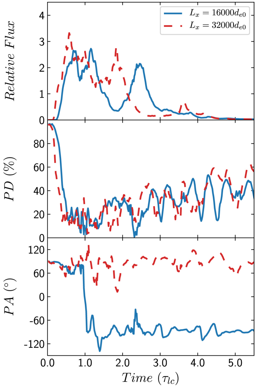
Figure 20. from Radiation and Polarization Signatures from Magnetic Reconnection in Relativistic Jets. I. A Systematic Study null 2020 APJ 901 149 doi:10.3847/1538-4357/abb1b0 https://dx.doi.org/10.3847/1538-4357/abb1b0 © 2020. The American Astronomical Society. All rights reserved.
