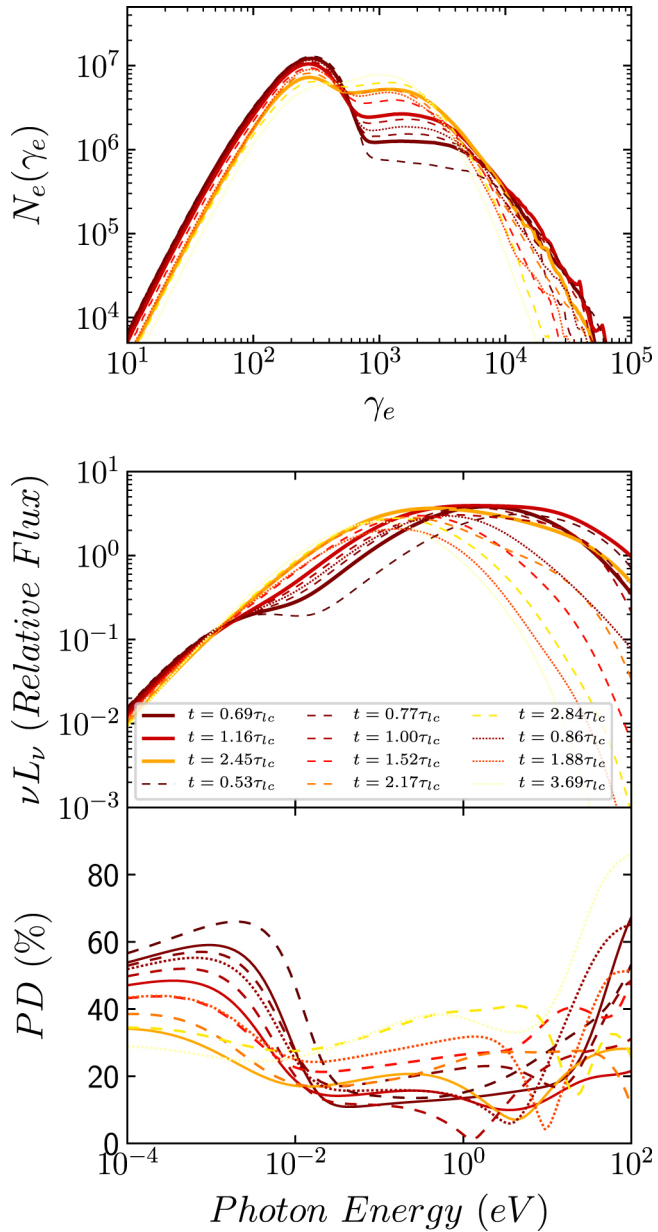
Figure 2. from Radiation and Polarization Signatures from Magnetic Reconnection in Relativistic Jets. I. A Systematic Study null 2020 APJ 901 149 doi:10.3847/1538-4357/abb1b0 https://dx.doi.org/10.3847/1538-4357/abb1b0 © 2020. The American Astronomical Society. All rights reserved.
