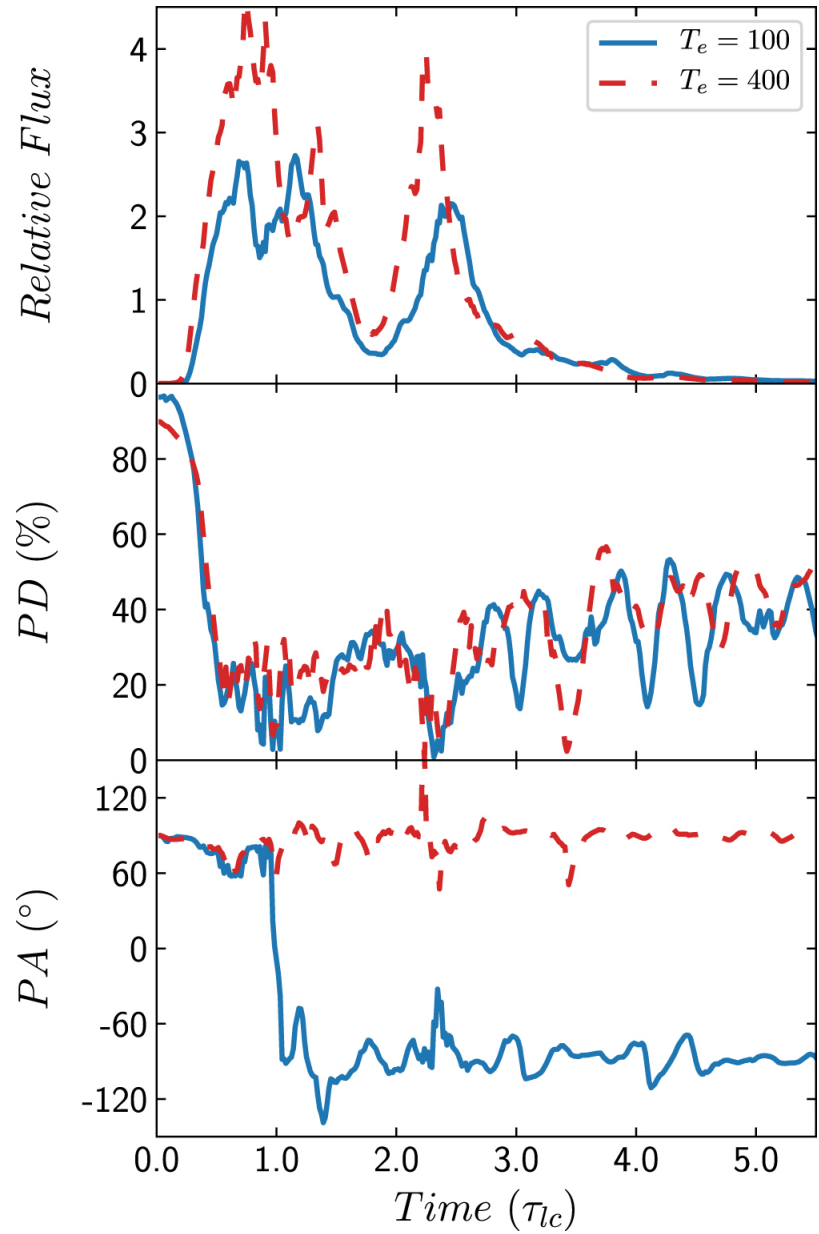
Figure 18. from Radiation and Polarization Signatures from Magnetic Reconnection in Relativistic Jets. I. A Systematic Study null 2020 APJ 901 149 doi:10.3847/1538-4357/abb1b0 https://dx.doi.org/10.3847/1538-4357/abb1b0 © 2020. The American Astronomical Society. All rights reserved.
