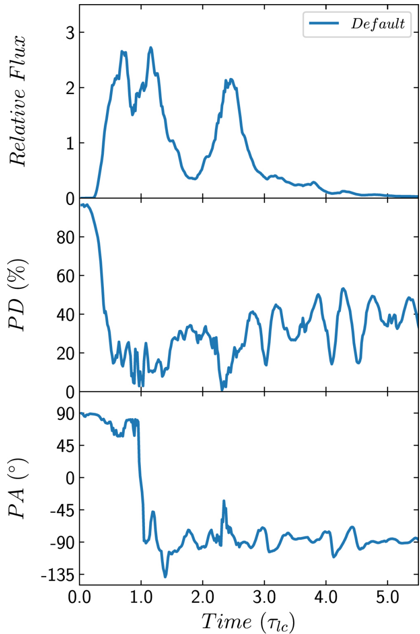
Figure 1. from Radiation and Polarization Signatures from Magnetic Reconnection in Relativistic Jets. I. A Systematic Study null 2020 APJ 901 149 doi:10.3847/1538-4357/abb1b0 https://dx.doi.org/10.3847/1538-4357/abb1b0 © 2020. The American Astronomical Society. All rights reserved.
