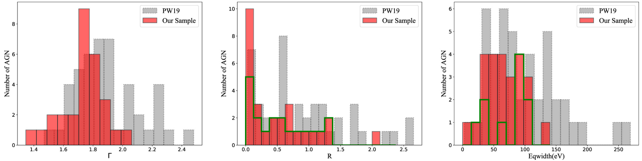
Figure 6. from NuSTAR Hard X-Ray Spectra of Radio Galaxies null 2020 APJ 901 111 doi:10.3847/1538-4357/abadf5 https://dx.doi.org/10.3847/1538-4357/abadf5 © 2020. The American Astronomical Society. All rights reserved.
