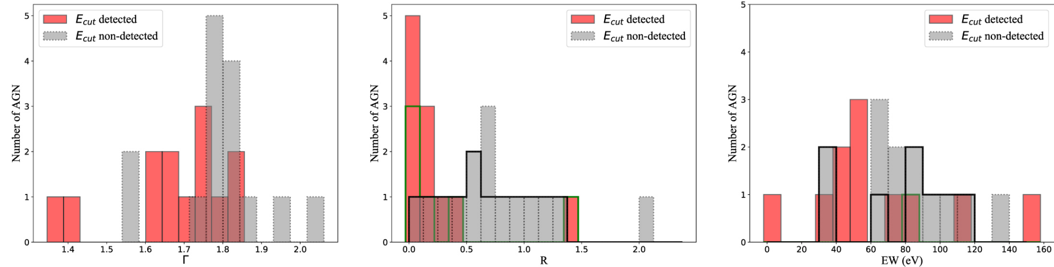
Figure 5. from NuSTAR Hard X-Ray Spectra of Radio Galaxies null 2020 APJ 901 111 doi:10.3847/1538-4357/abadf5 https://dx.doi.org/10.3847/1538-4357/abadf5 © 2020. The American Astronomical Society. All rights reserved.
