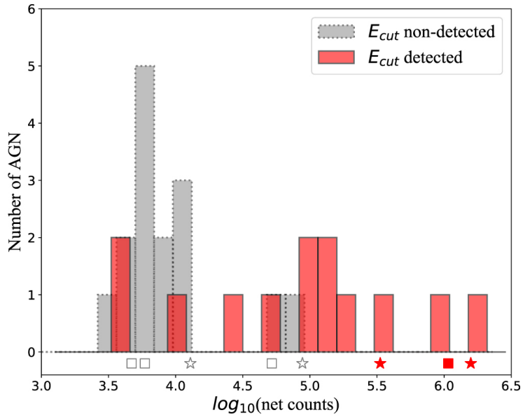
Figure 4. from NuSTAR Hard X-Ray Spectra of Radio Galaxies null 2020 APJ 901 111 doi:10.3847/1538-4357/abadf5 https://dx.doi.org/10.3847/1538-4357/abadf5 © 2020. The American Astronomical Society. All rights reserved.
