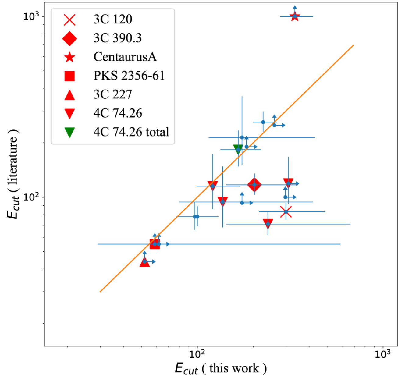
Figure 2. from NuSTAR Hard X-Ray Spectra of Radio Galaxies null 2020 APJ 901 111 doi:10.3847/1538-4357/abadf5 https://dx.doi.org/10.3847/1538-4357/abadf5 © 2020. The American Astronomical Society. All rights reserved.
