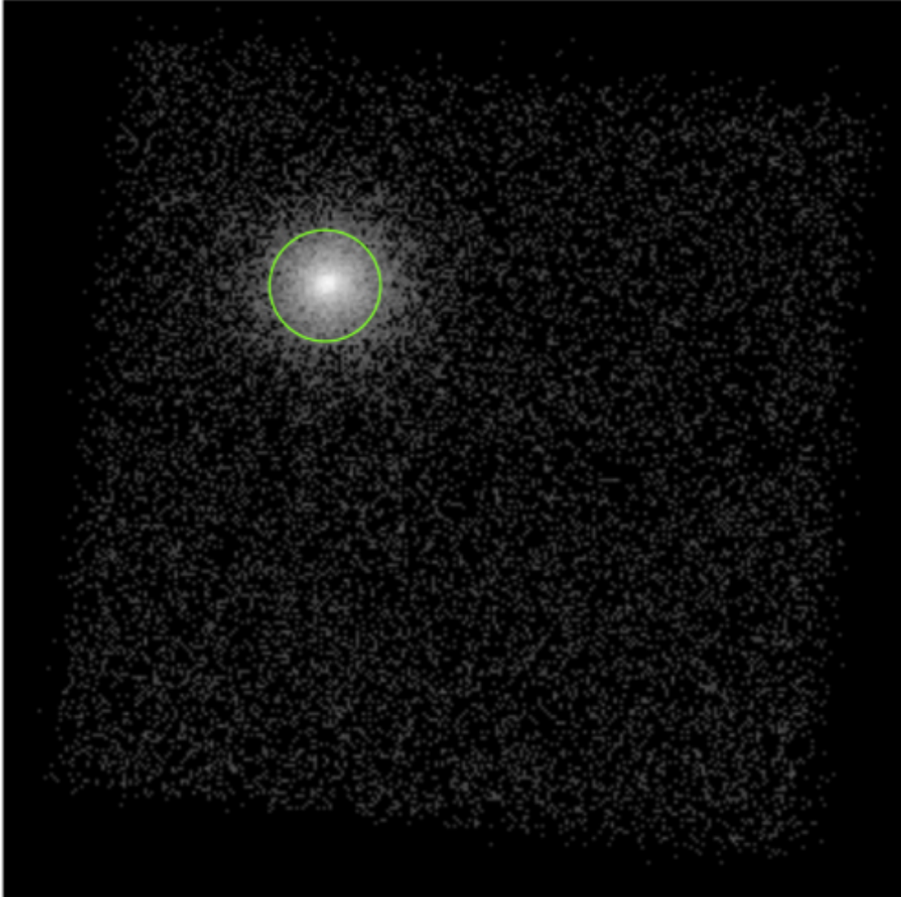
Figure 1. from NuSTAR Hard X-Ray Spectra of Radio Galaxies null 2020 APJ 901 111 doi:10.3847/1538-4357/abadf5 https://dx.doi.org/10.3847/1538-4357/abadf5 © 2020. The American Astronomical Society. All rights reserved.
