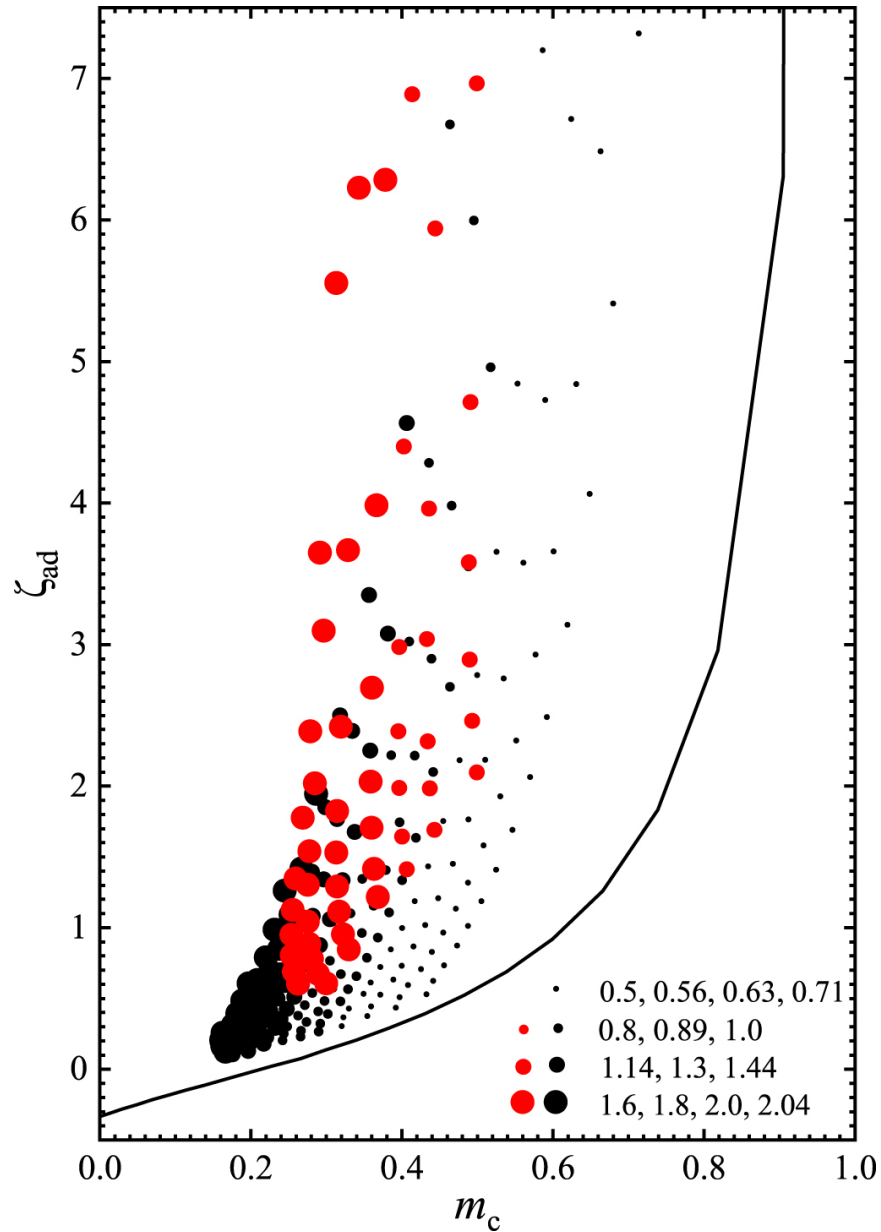
Figure 9. from Adiabatic Mass Loss in Binary Stars. III. From the Base of the Red Giant Branch to the Tip of the Asymptotic Giant Branch null 2020 APJ 899 132 doi:10.3847/1538-4357/aba7b7 https://dx.doi.org/10.3847/1538-4357/aba7b7 © 2020. The American Astronomical Society. All rights reserved.
