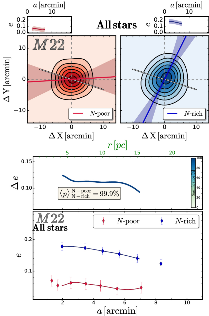
Figure 11. from Gaia and Hubble Unveil the Kinematics of Stellar Populations in the Type II Globular Clusters Centauri and M22 null 2020 APJ 898 147 doi:10.3847/1538-4357/aba04b https://dx.doi.org/10.3847/1538-4357/aba04b
