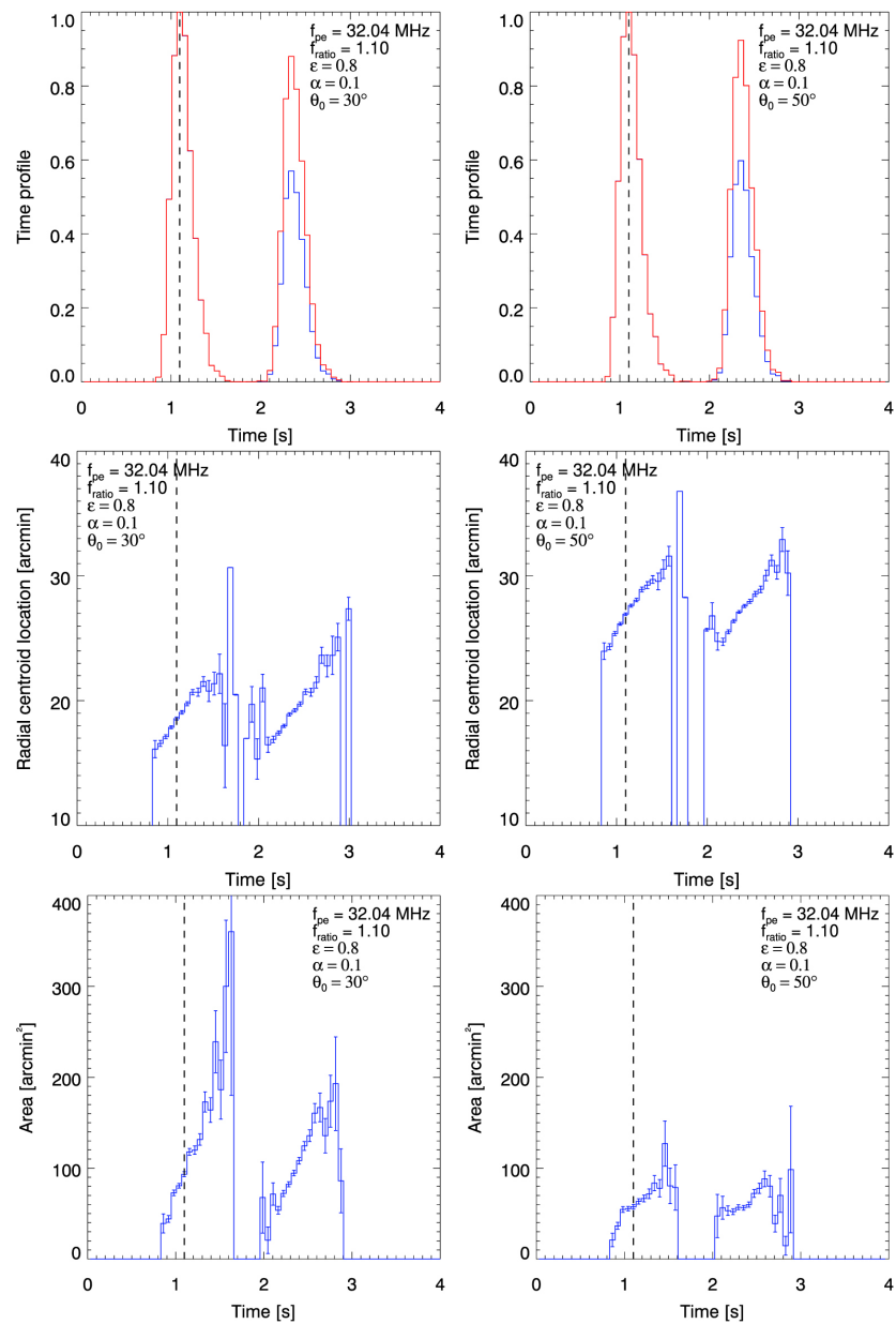
Figure 5. from Radio Echo in the Turbulent Corona and Simulations of Solar Drift-pair Radio Bursts null 2020 APJ 898 94 doi:10.3847/1538-4357/aba04a https://dx.doi.org/10.3847/1538-4357/aba04a
