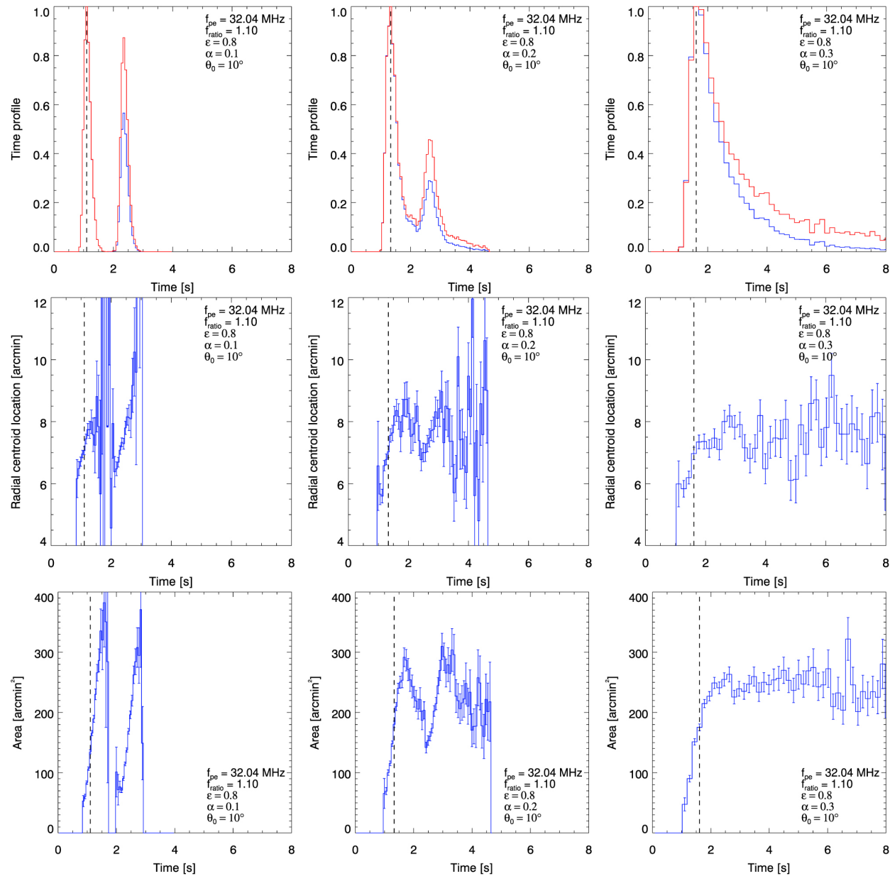
Figure 4. from Radio Echo in the Turbulent Corona and Simulations of Solar Drift-pair Radio Bursts null 2020 APJ 898 94 doi:10.3847/1538-4357/aba04a https://dx.doi.org/10.3847/1538-4357/aba04a
