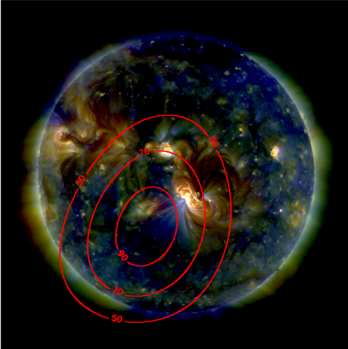
Figure 2. from Radio Echo in the Turbulent Corona and Simulations of Solar Drift-pair Radio Bursts null 2020 APJ 898 94 doi:10.3847/1538-4357/aba04a https://dx.doi.org/10.3847/1538-4357/aba04a © 2020. The Author(s). Published by the American Astronomical Society.
