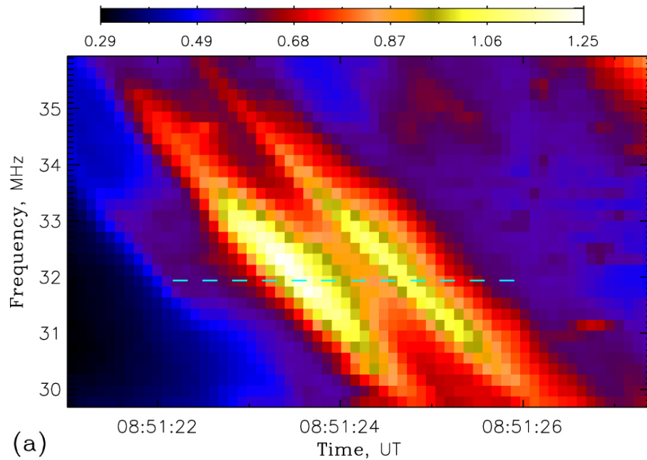
Figure 1. from Radio Echo in the Turbulent Corona and Simulations of Solar Drift-pair Radio Bursts null 2020 APJ 898 94 doi:10.3847/1538-4357/aba04a https://dx.doi.org/10.3847/1538-4357/aba04a © 2020. The Author(s). Published by the American Astronomical Society.
