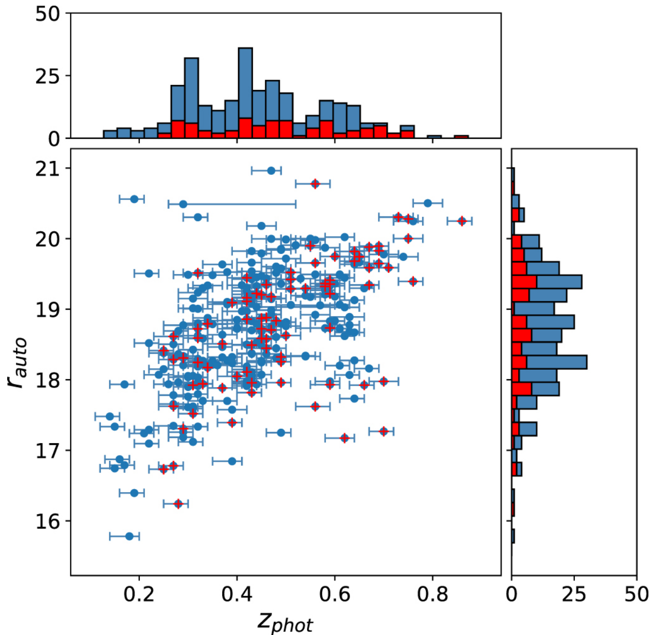
Figure 7. from New High-quality Strong Lens Candidates with Deep Learning in the Kilo-Degree Survey null 2020 APJ 899 30 doi:10.3847/1538-4357/ab9dfa https://dx.doi.org/10.3847/1538-4357/ab9dfa
