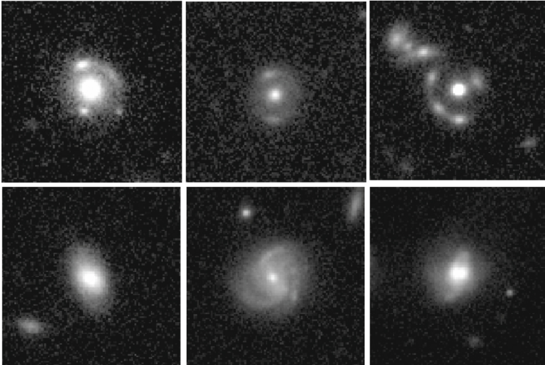
Figure 1. from New High-quality Strong Lens Candidates with Deep Learning in the Kilo-Degree Survey null 2020 APJ 899 30 doi:10.3847/1538-4357/ab9dfa https://dx.doi.org/10.3847/1538-4357/ab9dfa © 2020. The American Astronomical Society. All rights reserved.
