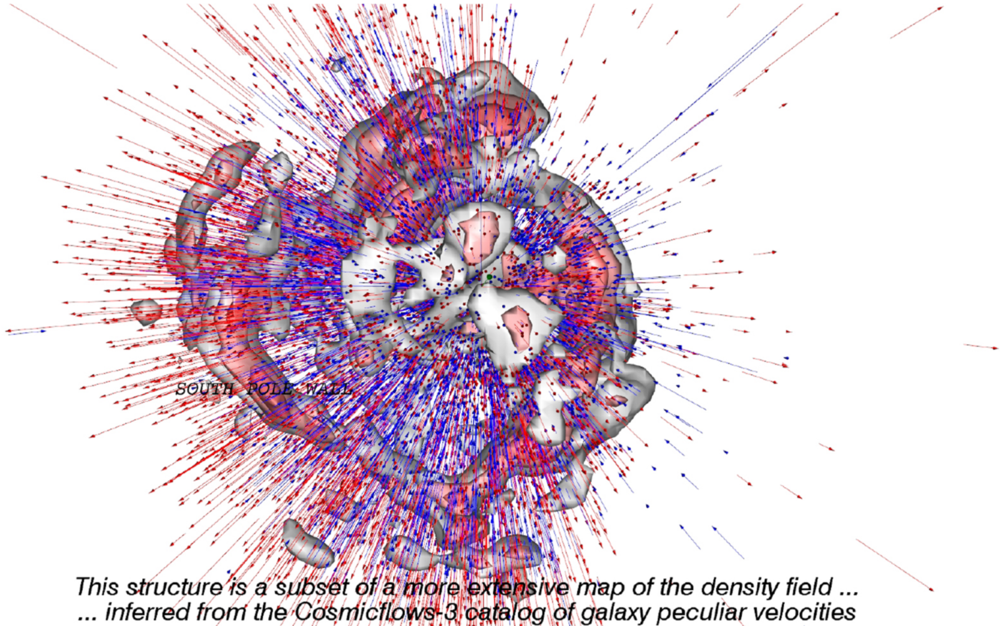
Figure 9. from Cosmicflows-3: The South Pole Wall null 2020 APJ 897 133 doi:10.3847/1538-4357/ab9952 https://dx.doi.org/10.3847/1538-4357/ab9952 © 2020. The American Astronomical Society. All rights reserved.
