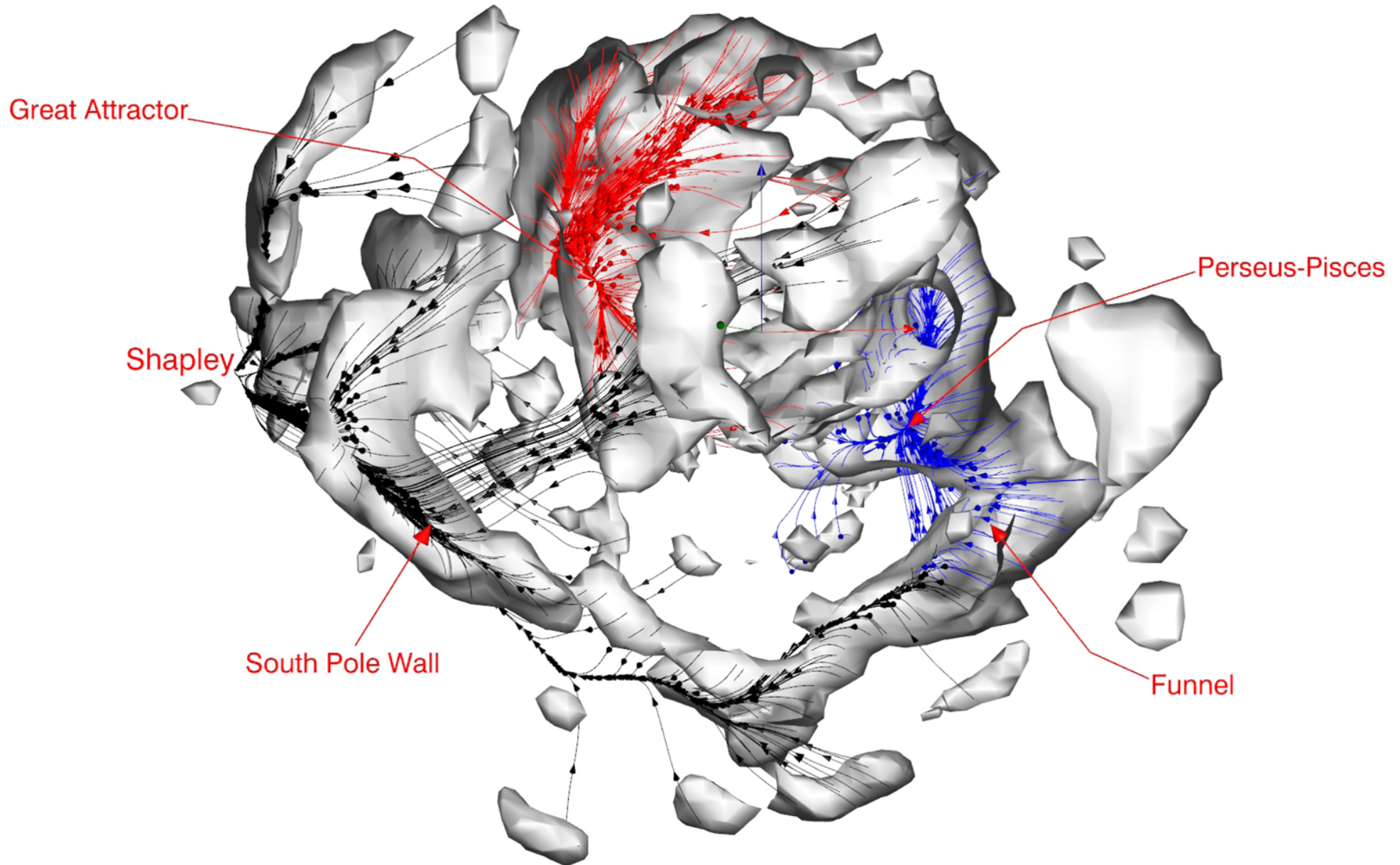
Figure 8. from Cosmicflows-3: The South Pole Wall null 2020 APJ 897 133 doi:10.3847/1538-4357/ab9952 https://dx.doi.org/10.3847/1538-4357/ab9952 © 2020. The American Astronomical Society. All rights reserved.
