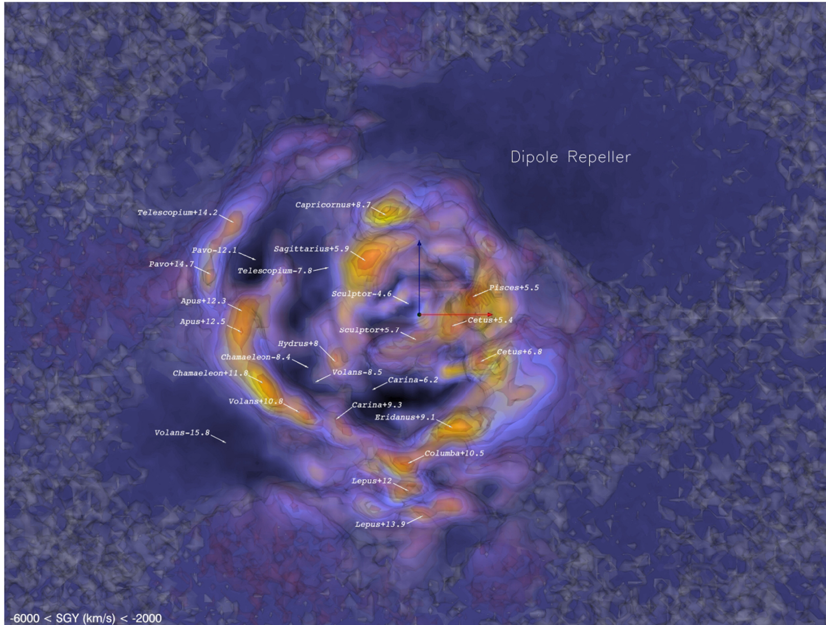
Figure 4. from Cosmicflows-3: The South Pole Wall null 2020 APJ 897 133 doi:10.3847/1538-4357/ab9952 https://dx.doi.org/10.3847/1538-4357/ab9952 © 2020. The American Astronomical Society. All rights reserved.
