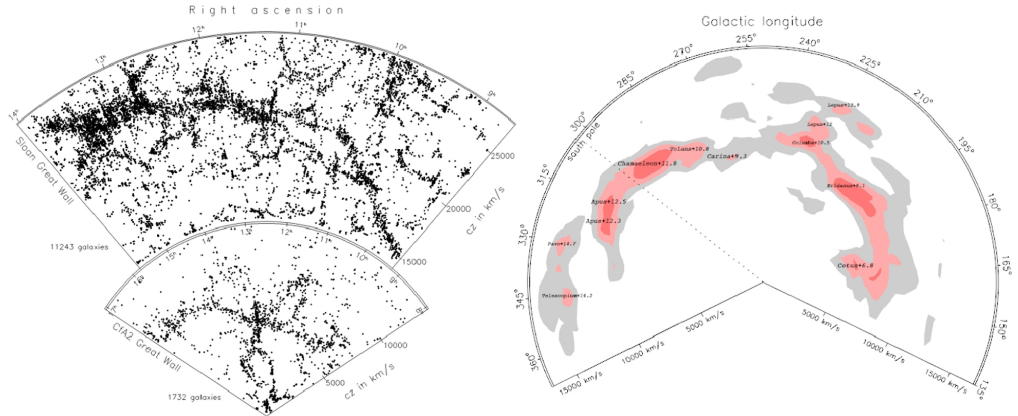
Figure 3. from Cosmicflows-3: The South Pole Wall null 2020 APJ 897 133 doi:10.3847/1538-4357/ab9952 https://dx.doi.org/10.3847/1538-4357/ab9952 © 2020. The American Astronomical Society. All rights reserved.
