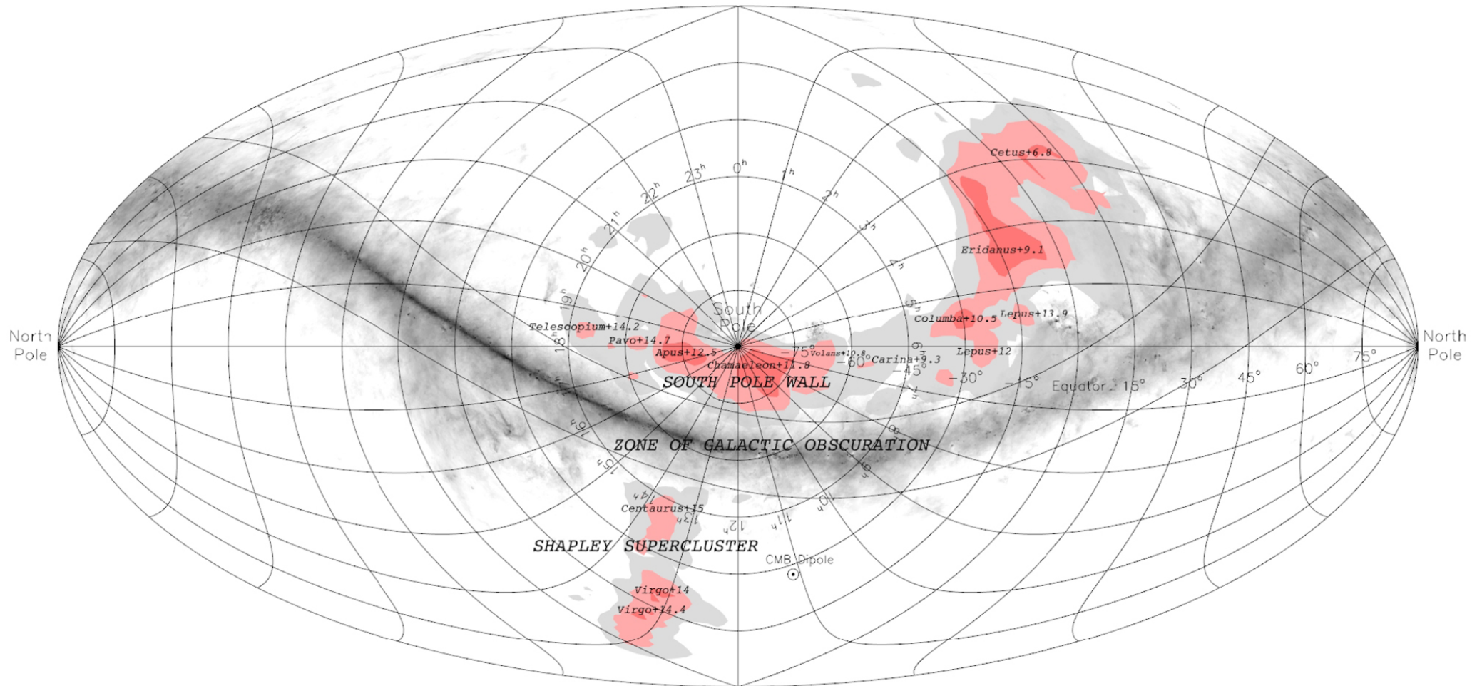
Figure 2. from Cosmicflows-3: The South Pole Wall null 2020 APJ 897 133 doi:10.3847/1538-4357/ab9952 https://dx.doi.org/10.3847/1538-4357/ab9952 © 2020. The American Astronomical Society. All rights reserved.
