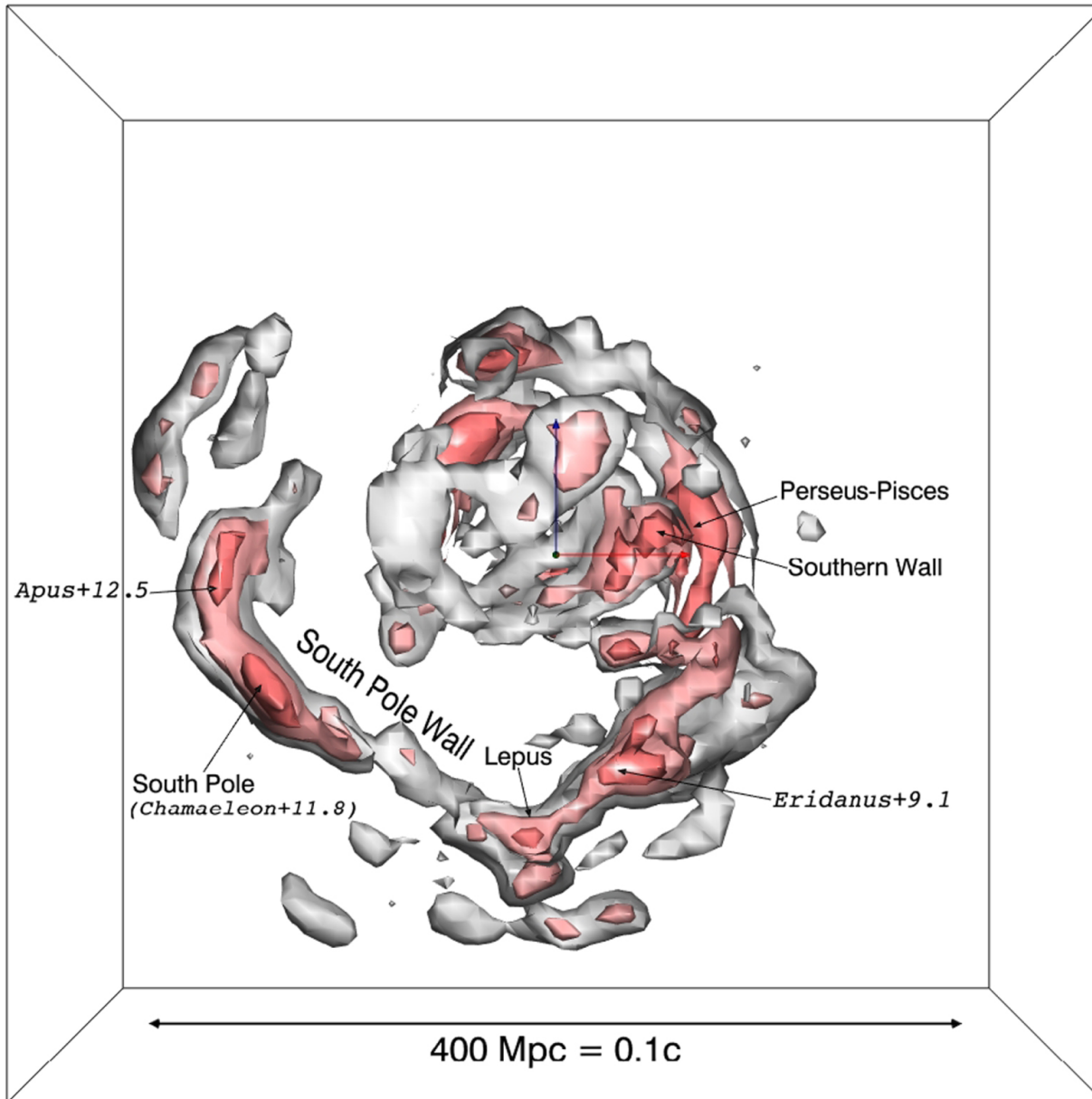
Figure 1. from Cosmicflows-3: The South Pole Wall null 2020 APJ 897 133 doi:10.3847/1538-4357/ab9952 https://dx.doi.org/10.3847/1538-4357/ab9952 © 2020. The American Astronomical Society. All rights reserved.
