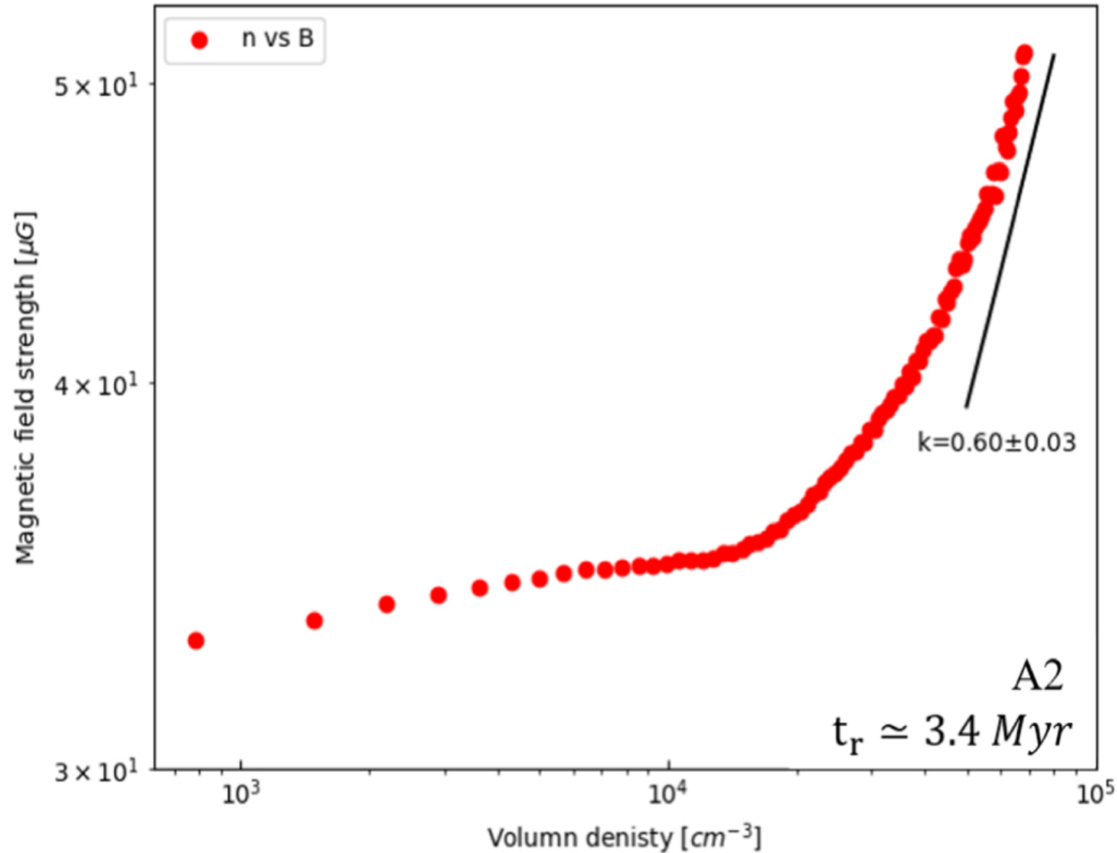
Figure 9. from Velocity Gradient in the Presence of Self-gravity: Identifying Gravity-induced Inflow and Determining Collapsing Stage null 2020 APJ 897 123 doi:10.3847/1538-4357/ab9948 https://dx.doi.org/10.3847/1538-4357/ab9948 © 2020. The American Astronomical Society. All rights reserved.
