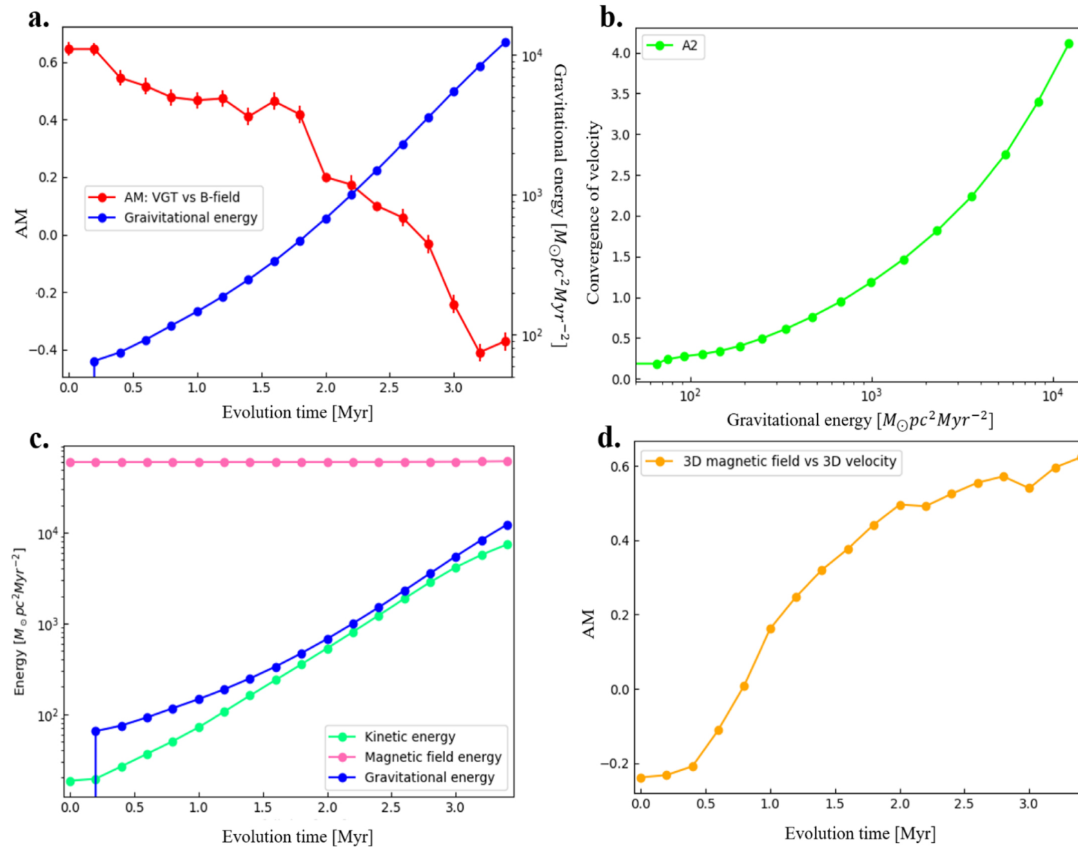
Figure 7. from Velocity Gradient in the Presence of Self-gravity: Identifying Gravity-induced Inflow and Determining Collapsing Stage null 2020 APJ 897 123 doi:10.3847/1538-4357/ab9948 https://dx.doi.org/10.3847/1538-4357/ab9948 © 2020. The American Astronomical Society. All rights reserved.
