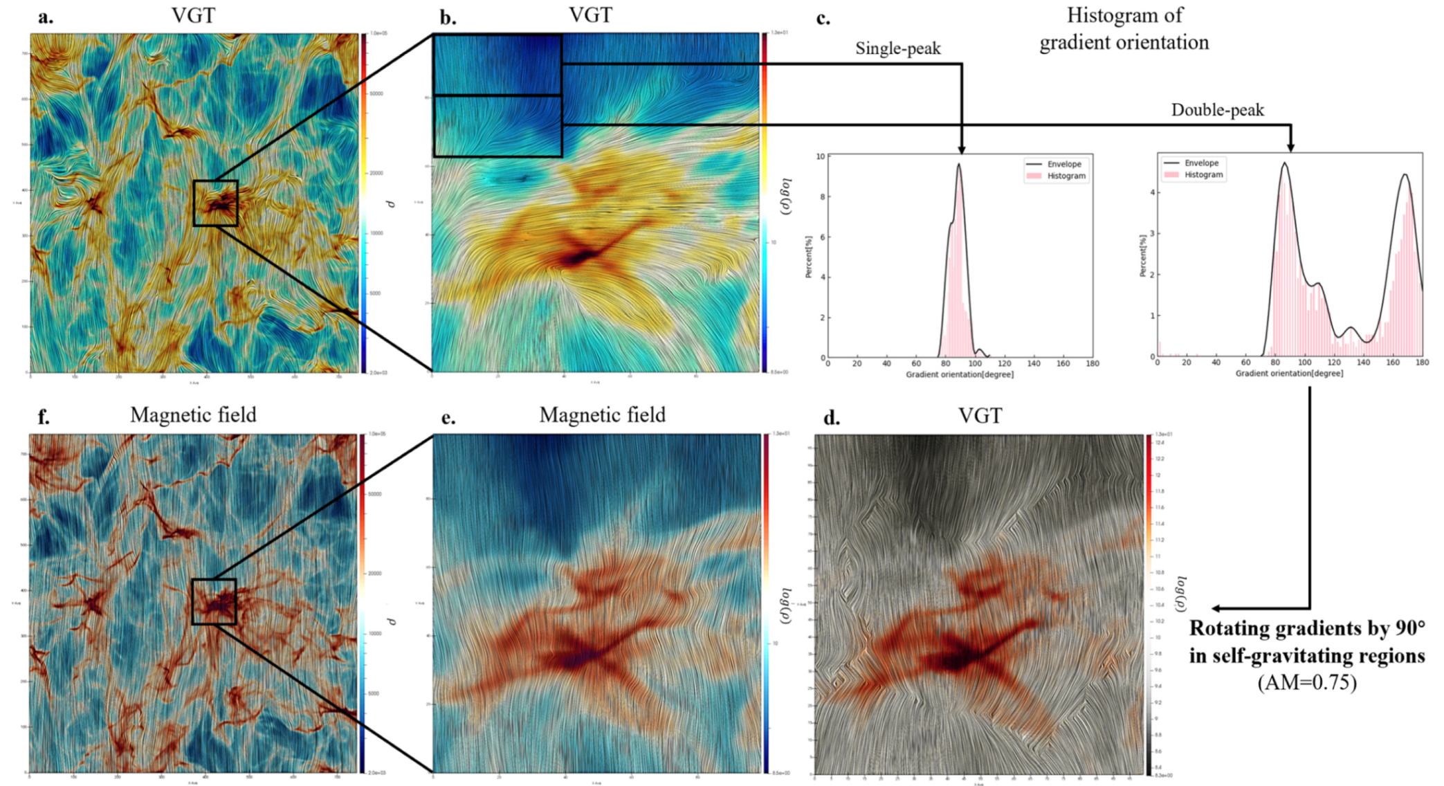
Figure 4. from Velocity Gradient in the Presence of Self-gravity: Identifying Gravity-induced Inflow and Determining Collapsing Stage null 2020 APJ 897 123 doi:10.3847/1538-4357/ab9948 https://dx.doi.org/10.3847/1538-4357/ab9948 © 2020. The American Astronomical Society. All rights reserved.
