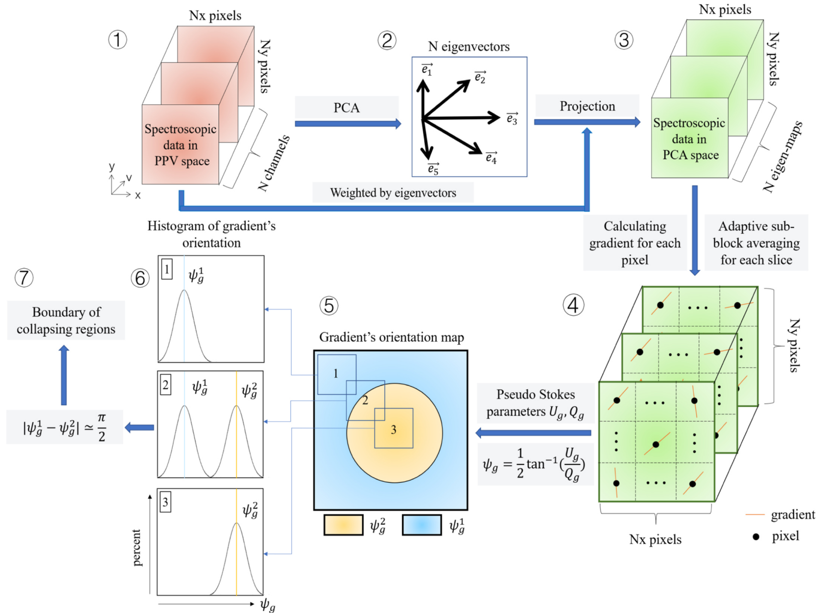
Figure 3. from Velocity Gradient in the Presence of Self-gravity: Identifying Gravity-induced Inflow and Determining Collapsing Stage null 2020 APJ 897 123 doi:10.3847/1538-4357/ab9948 https://dx.doi.org/10.3847/1538-4357/ab9948 © 2020. The American Astronomical Society. All rights reserved.
