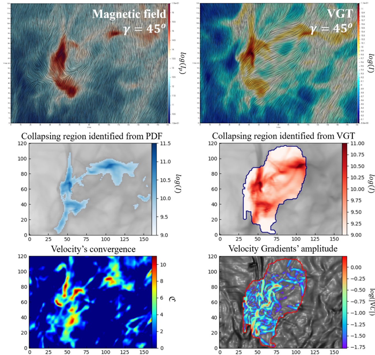
Figure A2. from Velocity Gradient in the Presence of Self-gravity: Identifying Gravity-induced Inflow and Determining Collapsing Stage null 2020 APJ 897 123 doi:10.3847/1538-4357/ab9948 https://dx.doi.org/10.3847/1538-4357/ab9948 © 2020. The American Astronomical Society. All rights reserved.
